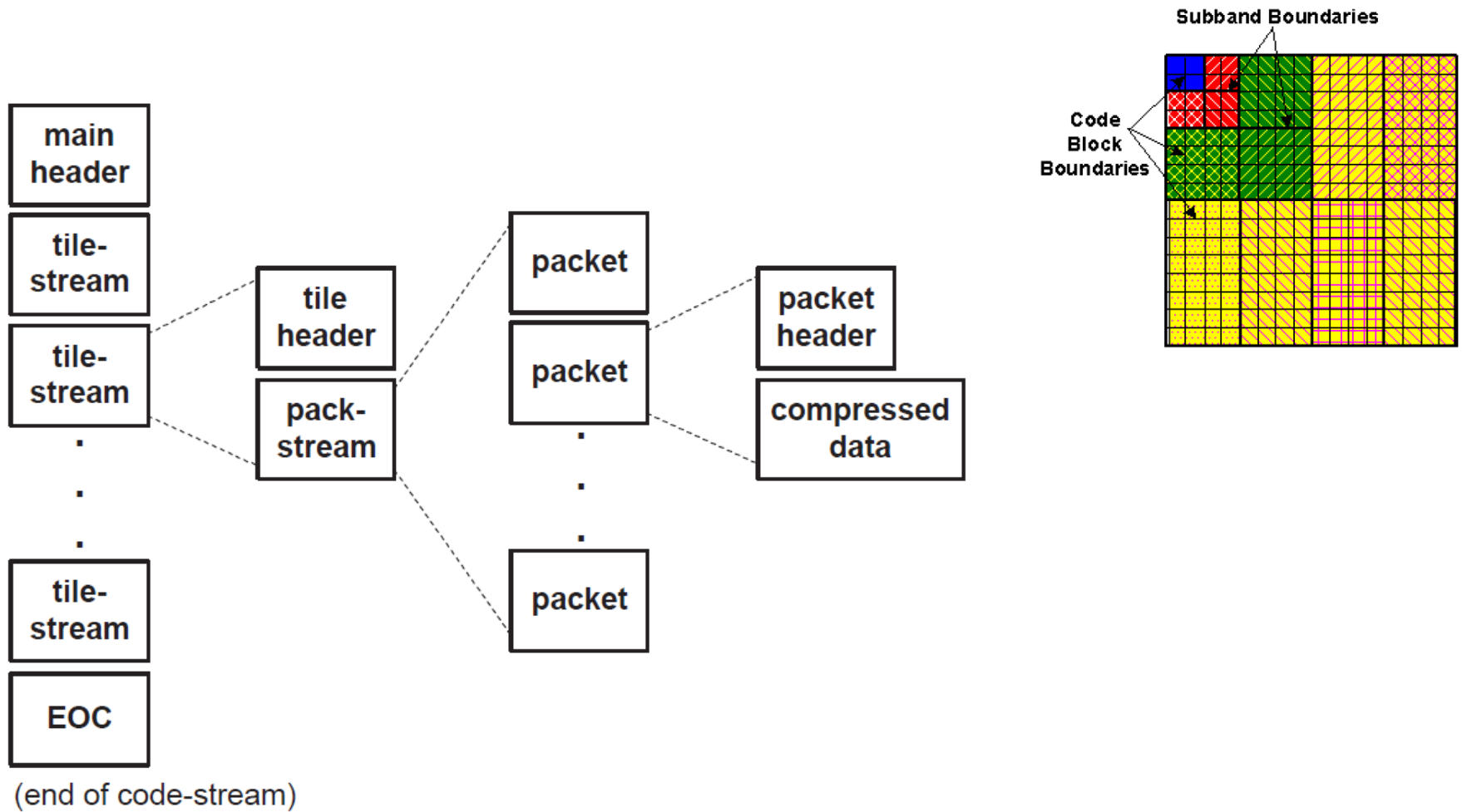
Figure 20: Code-stream organization [1].
