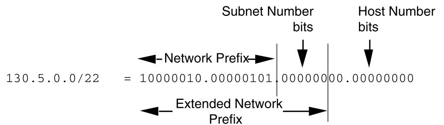
FIGURE 16. 130.5.0/16 with a /22 Extended Network Prefix
