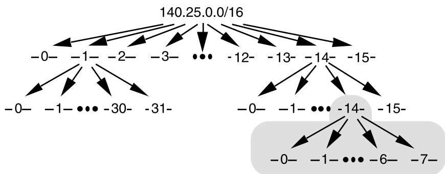
FIGURE 26. Sub-Subnets for Subnet #14-14 (140.25.238.0/24)
