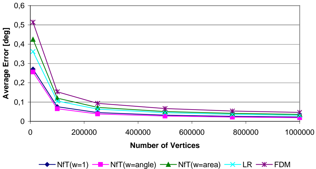
Graph 2: The estimation errors for f_2(x, y) = x^2 + 0.25 \cdot \sin(2 \cdot \pi \cdot y)
