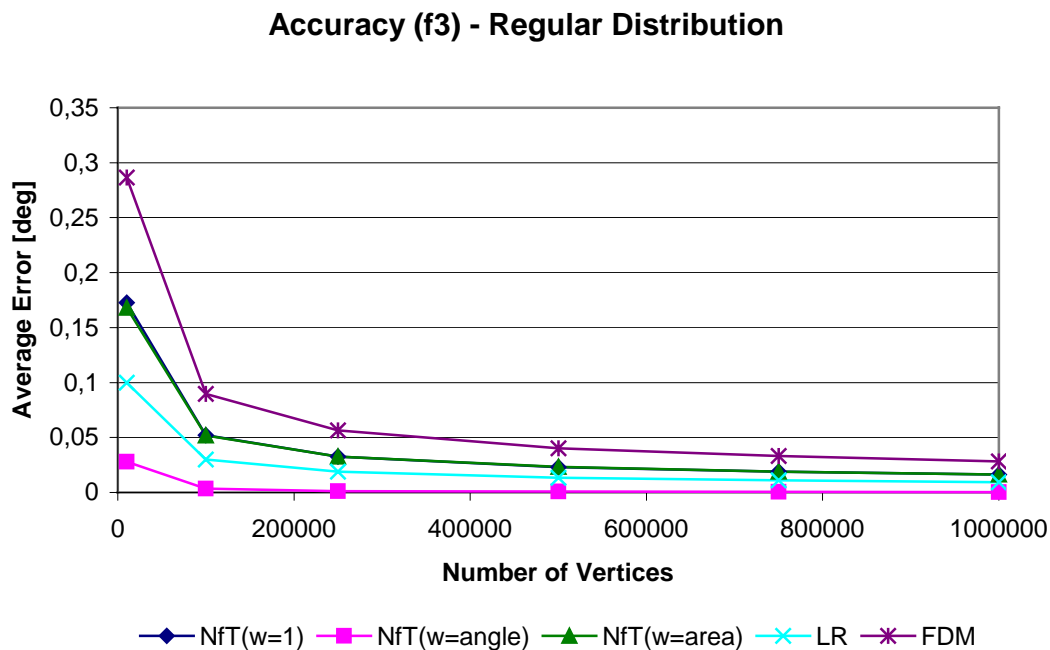
Graph 6: Estimation from meshes with regular vertex distribution.
